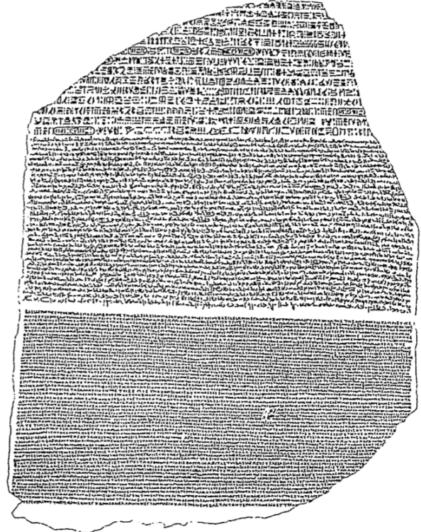
Rosetta Stone
